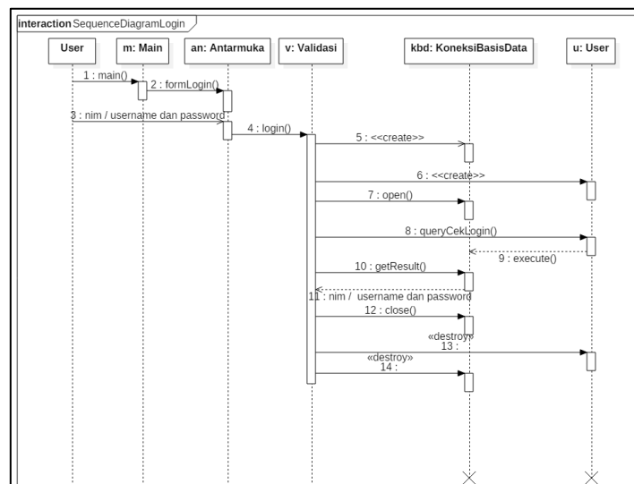
Gambar 6. Sequence diagram sistem
