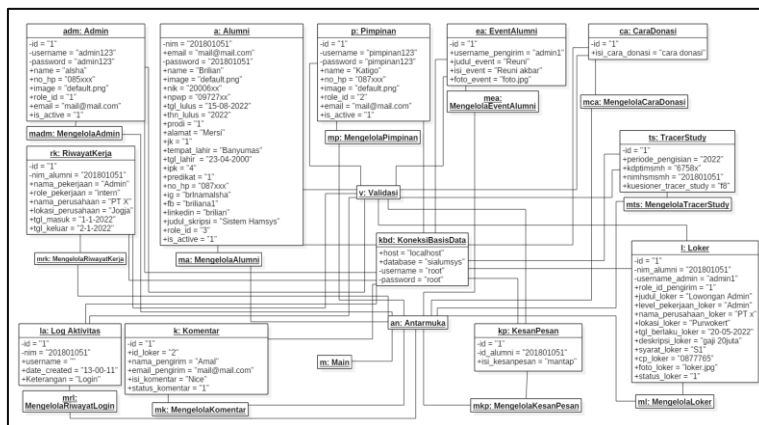
Gambar 4. Object diagram sistem
