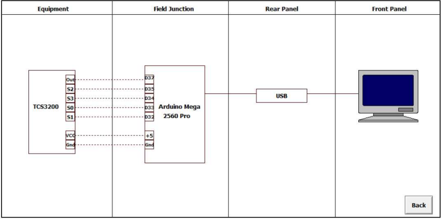
Gambar 10 Loop diagram pendeteksi warna
