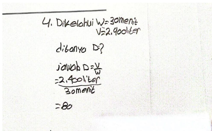
Figure 4. Conclusion Error
