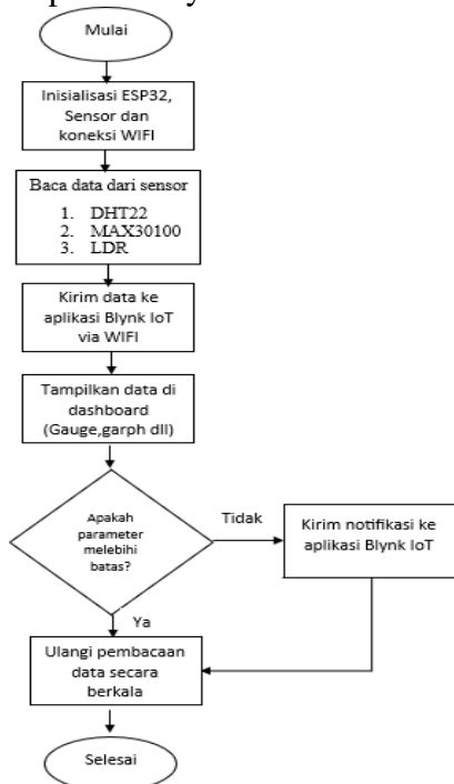
Gambar2. 3 Flowchart system
