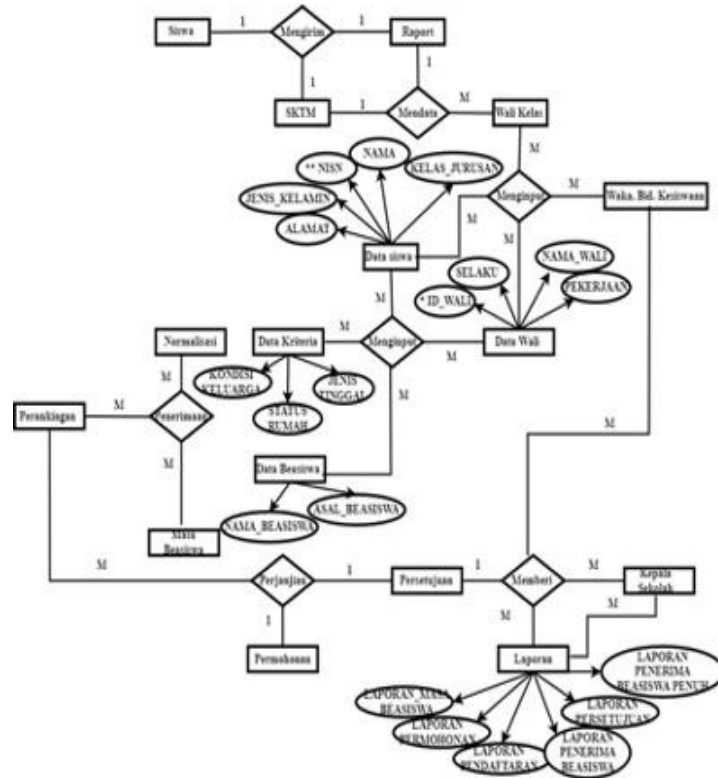
Gambar 5. Entity Diagram Relationship
