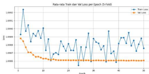
Gambar 6 Grafik Rata-Rata Train Loss Dan Val Loss Optimizer
