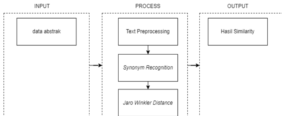
Gambar 1 Diagram IPO
