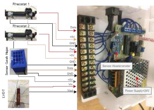
Figure 5. Circuit of Land shift Detection System
