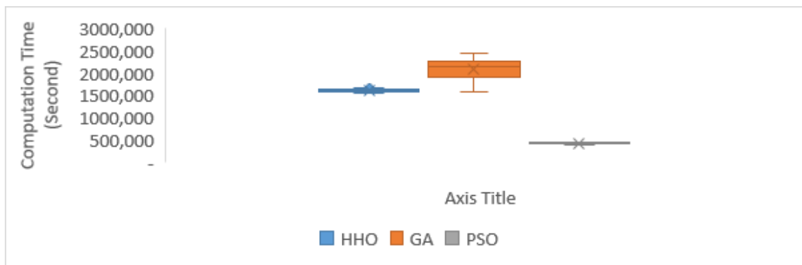
Figure 9. Boxplot of computation time for each algorithm in Case 1.
