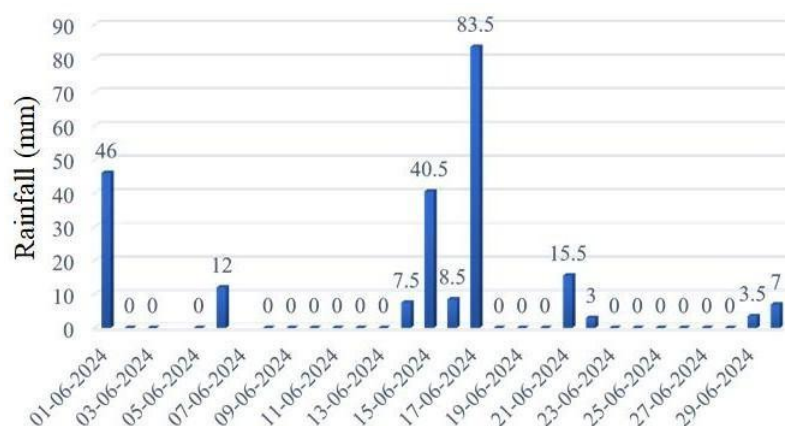
Figure 7. Rainfall (mm) in June 2024
