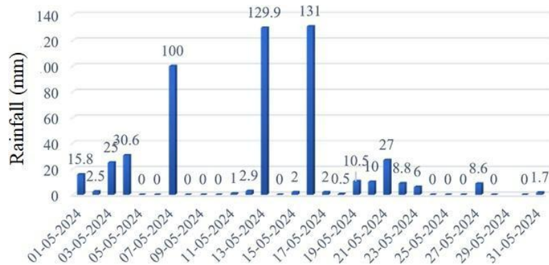
Figure 6. Rainfall (mm) in May 2024
