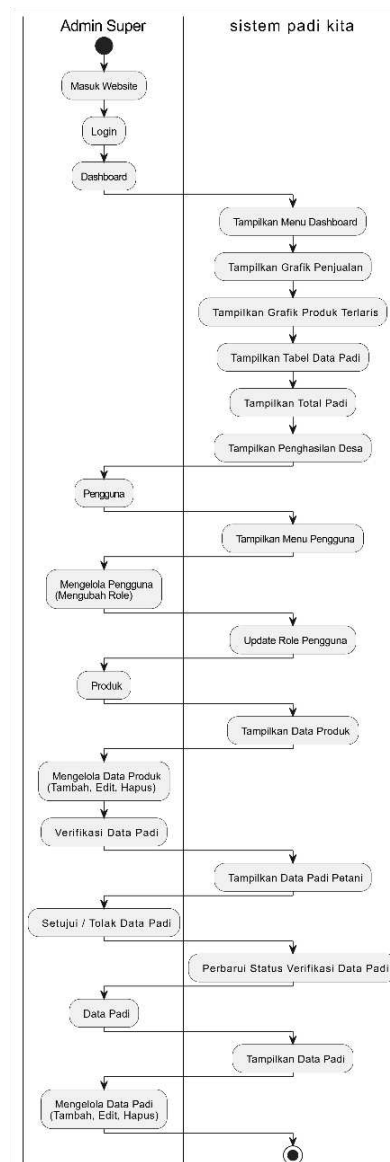
Gambar 3. Activity Diagram
