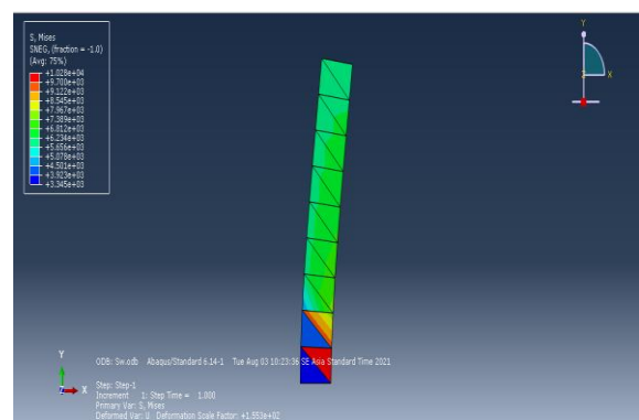
Gambar 4. Kontur Tegangan Free standing shear wall
