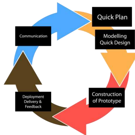
Gambar 2. Siklus Prototype [2]
