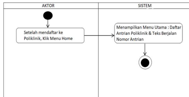
Gambar 11. Activity Diagram Nomor Antrian
