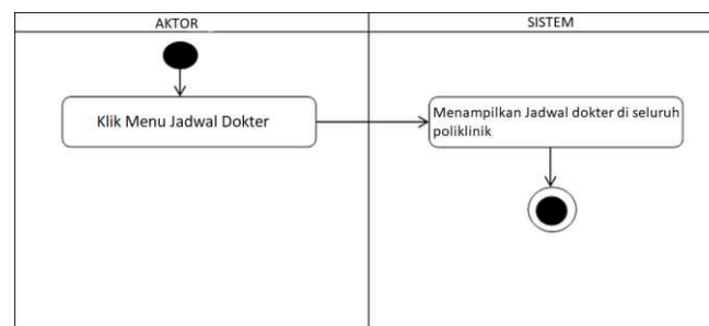
Gambar 8. Activity Diagram Jadwal Dokter
