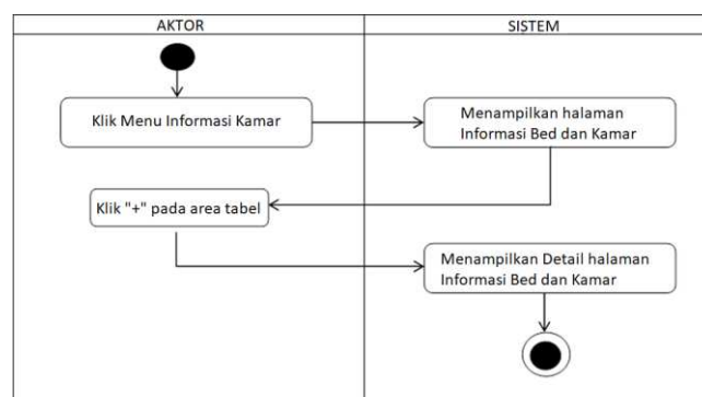
Gambar 9. Activity Diagram Informasi Kamar
