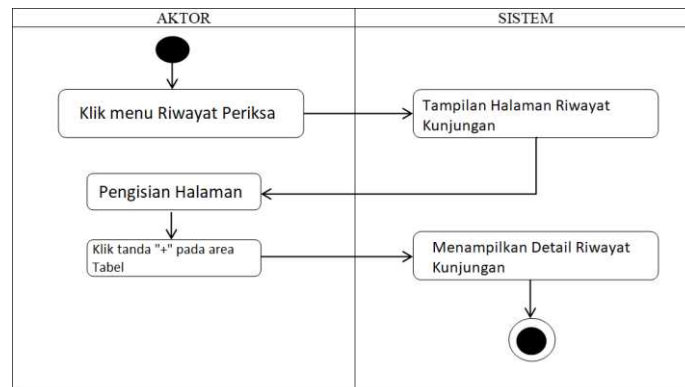
Gambar 7. Activity Diagram Riwayat Kunjungan
