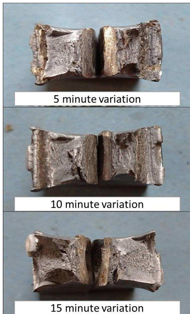
Figure 6. Impact test results for each welding speed variation The impact test results data is in Table 3 below.
