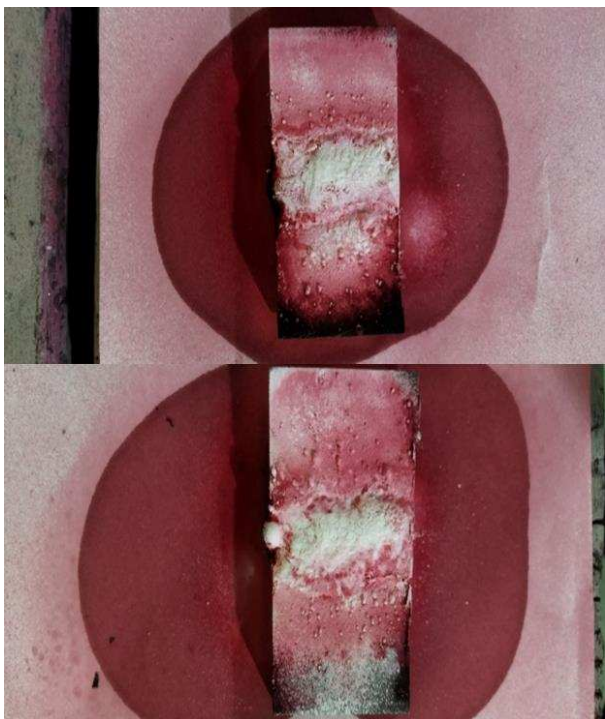
Figure 5. Data from observations using red dye penetrant on impact test specimens.
