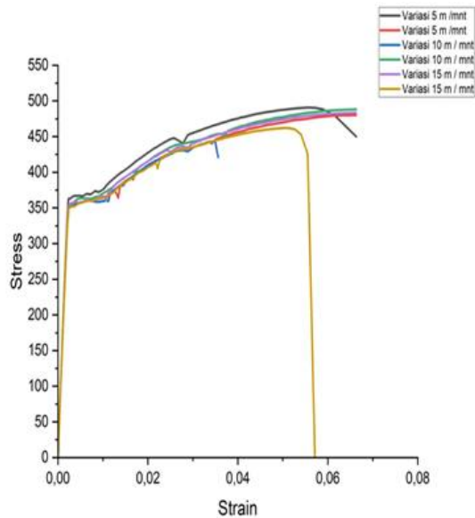
Figure 10. Combined Tensile Test Graph
