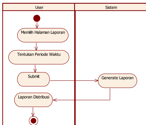
Gambar 4. Laporan Distribusi Telur
