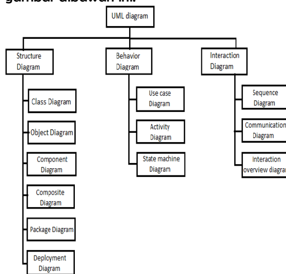
Gambar 1. Diagram UML
