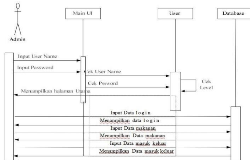
Gambar 5. Sequence Diagram
