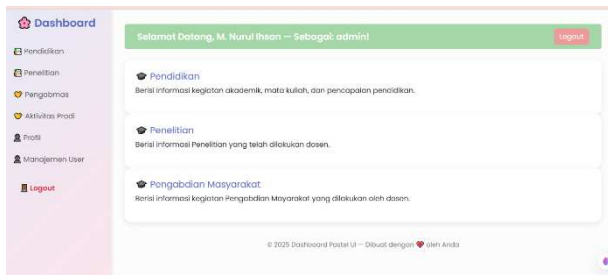
Figure 4. Dashboard page
