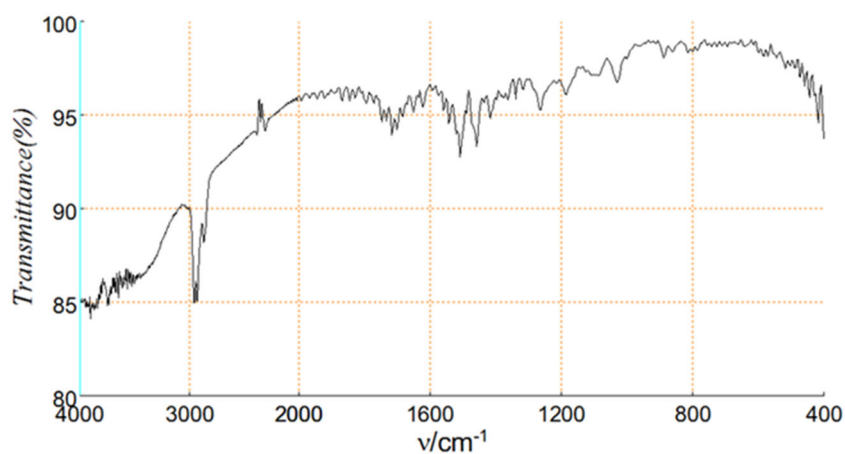
Fig S21. FTIR spectrum of 7-hydroxycalamenene (2)
