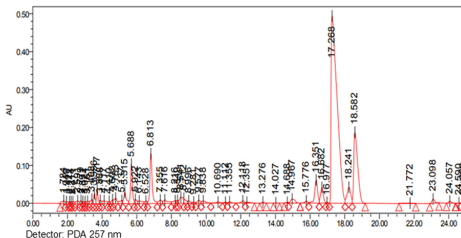
Fig S1. HPLC chromatogram for compounds 1 and 2
