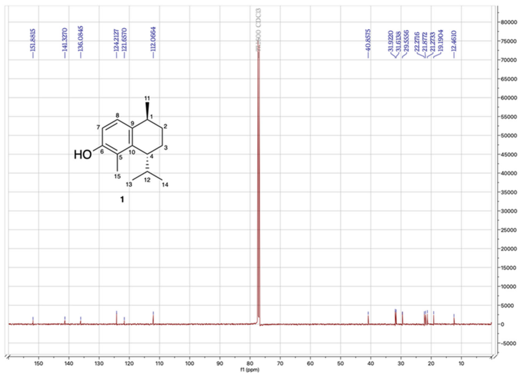
Fig S3. ^{13}\text{C} -NMR spectrum (150 MHz) of dysoxyphenol (1) in \text{CDCl}_3
