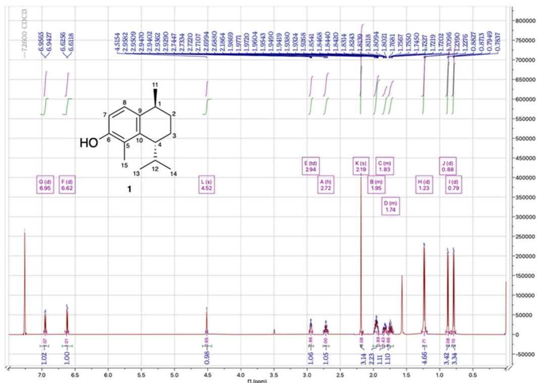
Fig S2. ^1\text{H} -NMR spectrum (600 MHz) of dysoxyphenol (1) in \text{CDCl}_3
