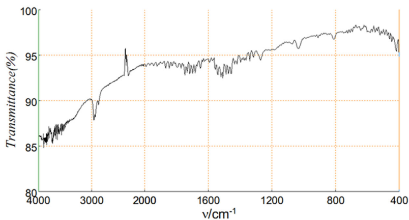
Fig S11. FTIR spectrum of dysoxyphenol (1)
