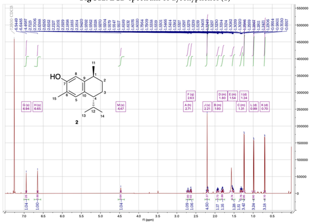
Fig S13. ^1\text{H} (600 MHz) NMR spectrum of 7-hydroxycalamenene (2) in \text{CDCl}_3
