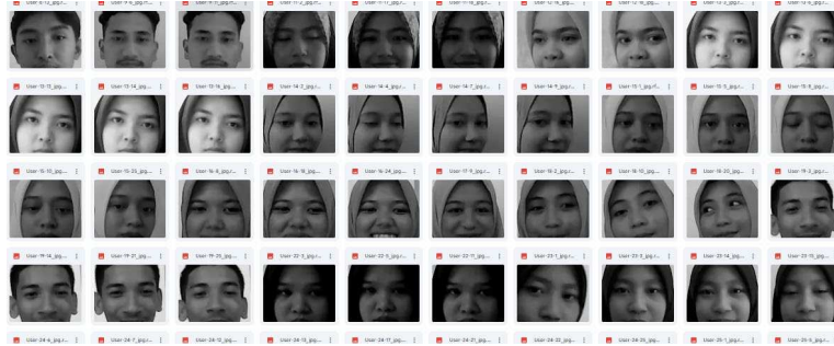
Gambar 3.7 data Testing
