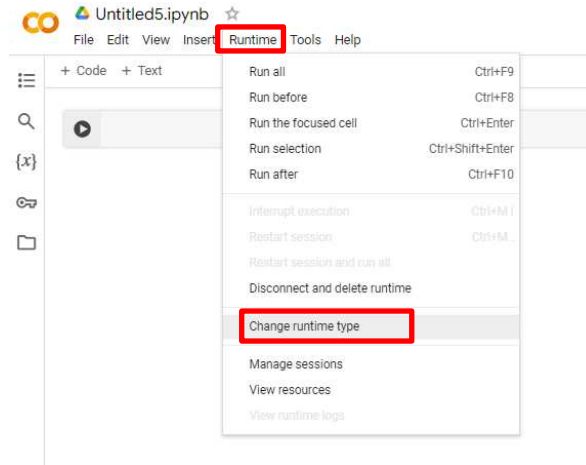
Gambar 4.4 Runtime
