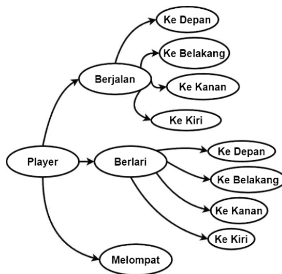
Gambar 4. FSM Player
