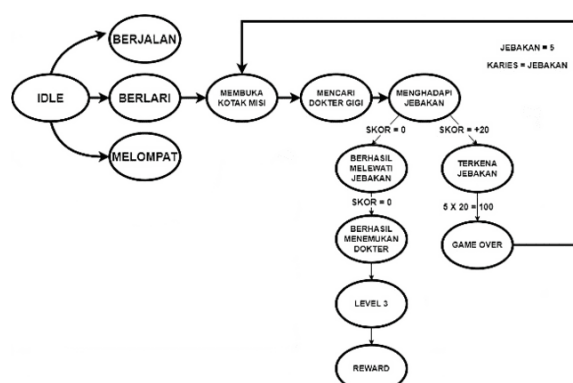
Gambar 6. FSM Level 2
