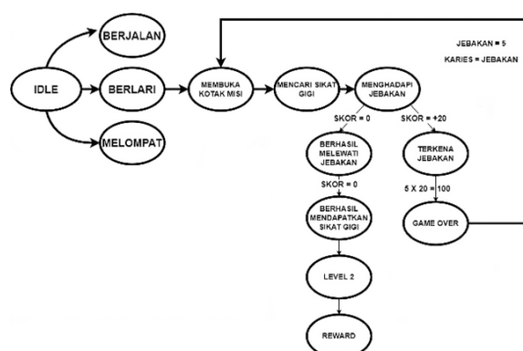
Gambar 5. FSM Level 1
