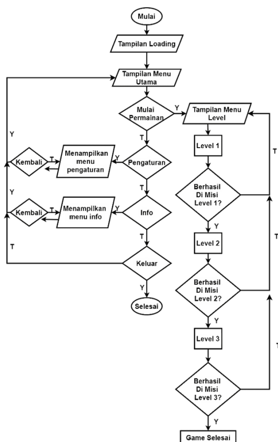
Gambar 2. Flowchart Game
