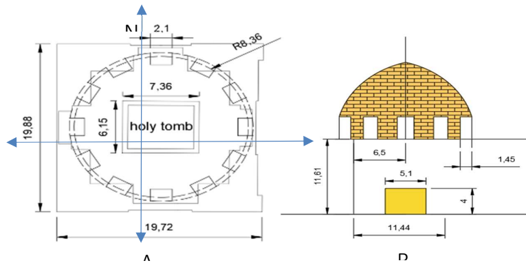
Figure 13. Geometrical dimensions of the study place, A: the plan view and B: the cross-section view.
