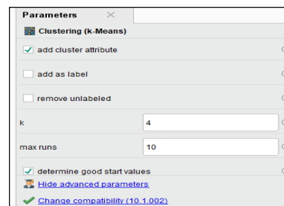
Figure 3. Rapidminer's Configuration
