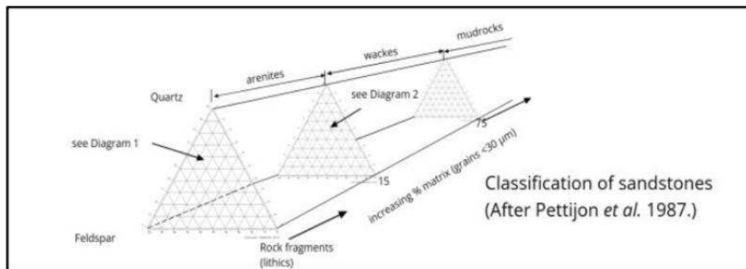
Diagram 2 Wackes*
