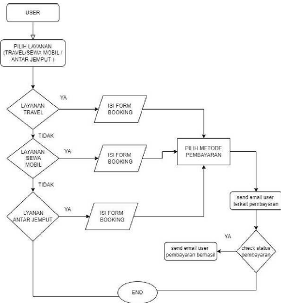
Gambar 4. Flowchart proses bisnis
