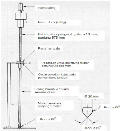
Gambar 4 Alat Dynamic Cone Penetrometer (DCP).
