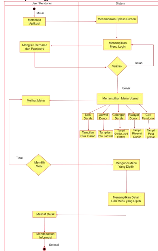
Gambar 4. Activity Diagram User
