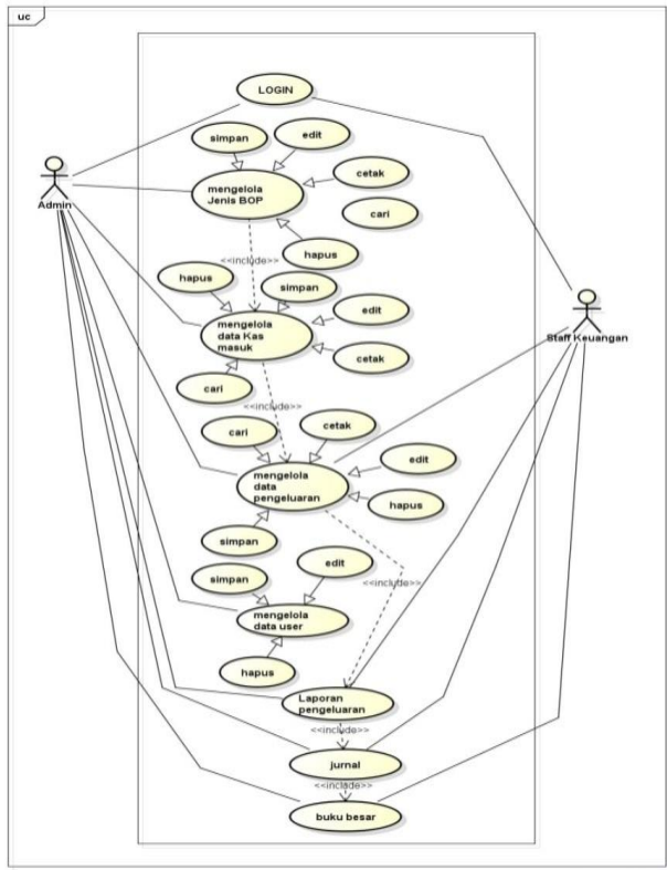
Gambar 3. Usecase Diagram
