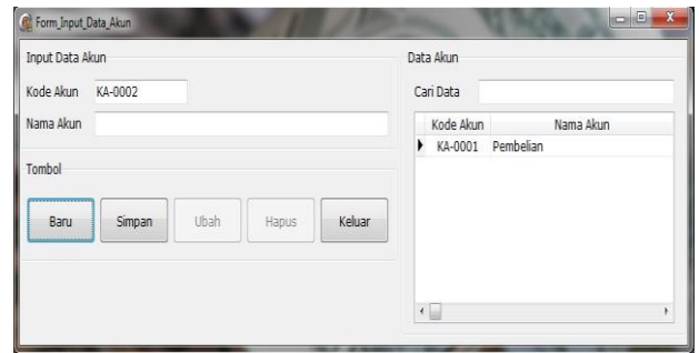
Gambar 4. Form BOP
