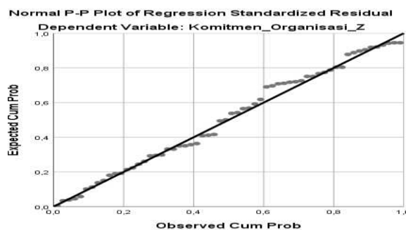
Figure 1. PP Plot Sub 1
