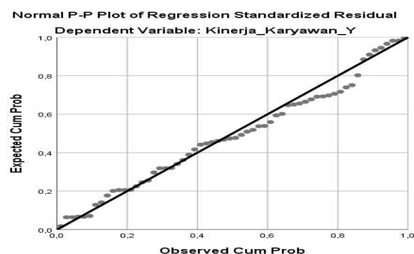
Figure 2. PP Plot Sub 2
