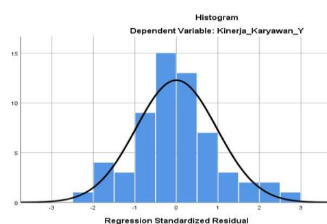
Figure 4. Sub 2 histogram
