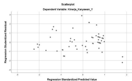
Figure 6. Sub 2 Heteroscedasticity Test Results
