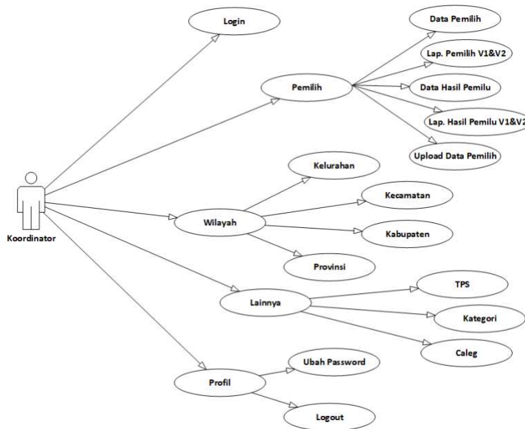
Gambar 3. Use Case Diagram Koordinator
