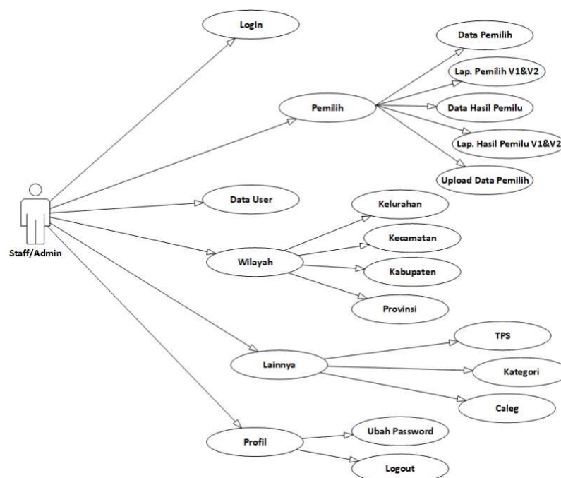
Gambar 2. Use Case Diagram Staf/Admin
