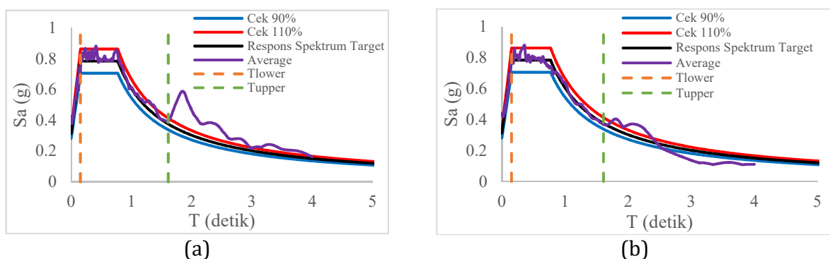
Gambar 4. (a) Kontrol rata-rata pseudo acceleration spektrum arah X, (b) Kontrol rata-rata pseudo acceleration spektrum arah Y
